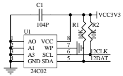
MEMORY
