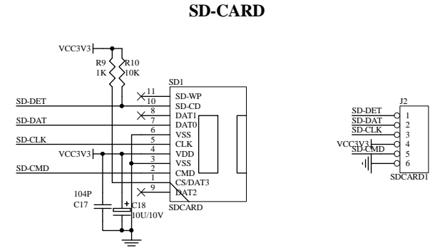
SD-CARD
