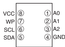
8-ball dBGA2
