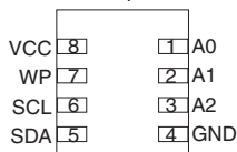
8-lead Ultra Thin Mini-MAP (MLP 2x3)
