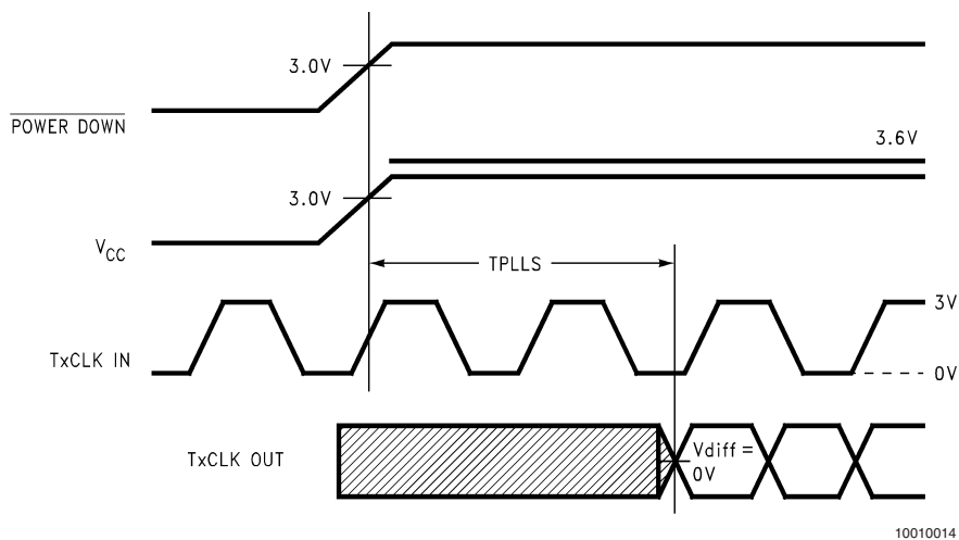
FIGURE 8. DS90C383A/DS90CF383A (Transmitter) Phase Lock Loop Set Time
