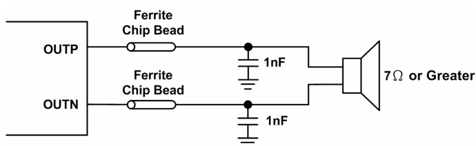
Figure 15. Typical Ferrite Chip Bead Filter
