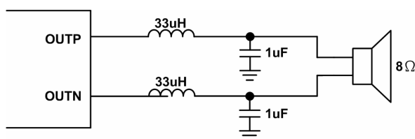
Figure 16. Typical LC Output Ferrite for 8Ω Speaker
