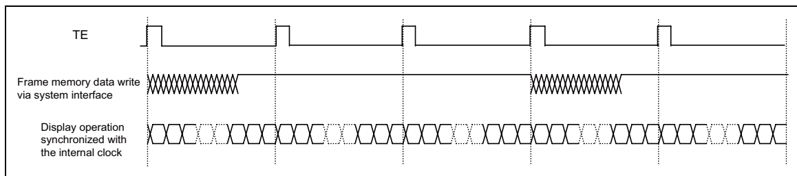
Figure 72 Video Image Data Write with TE
