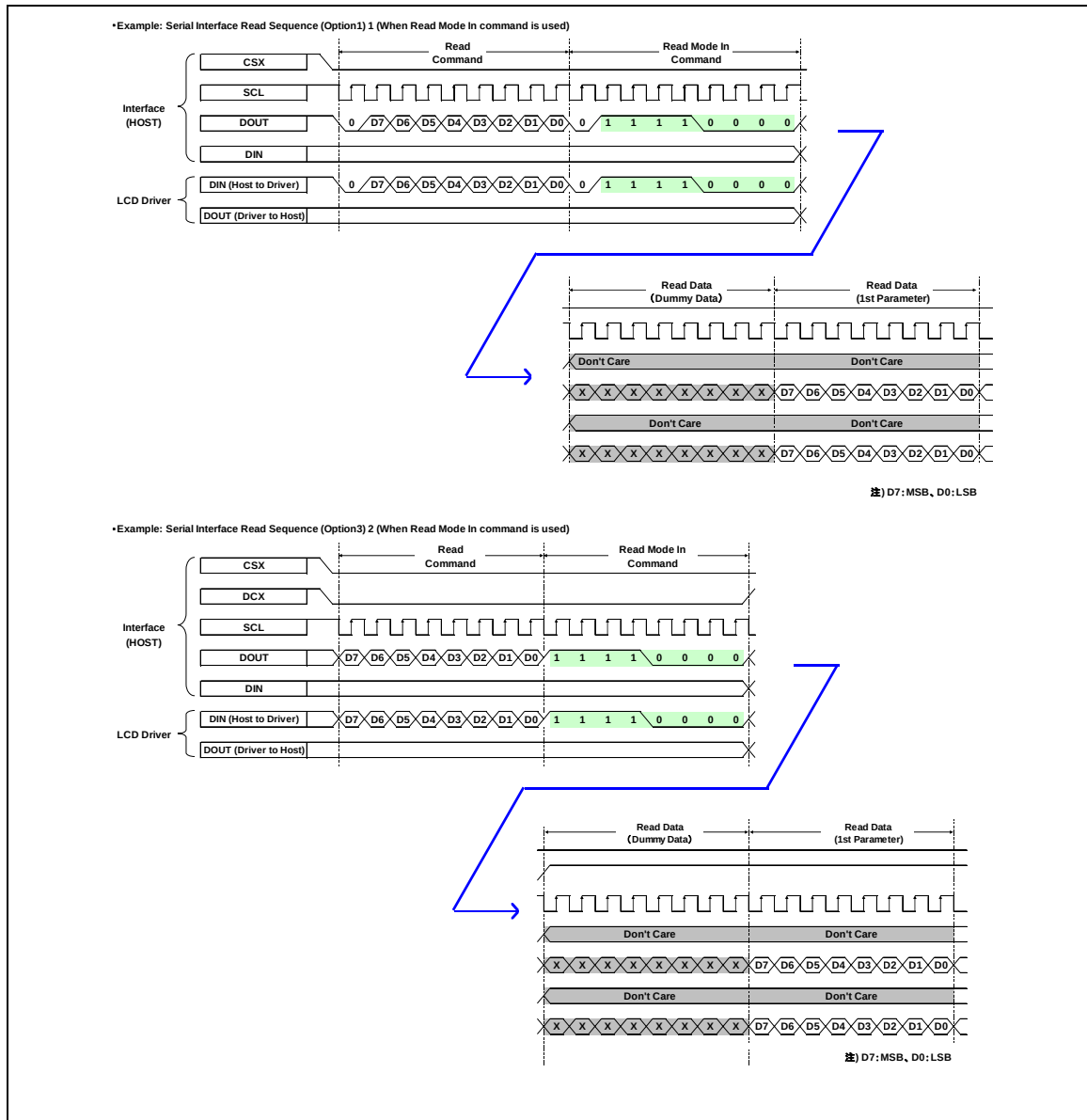
Figure 18 Serial Interface Read Cycle Sequence (Example 2)
