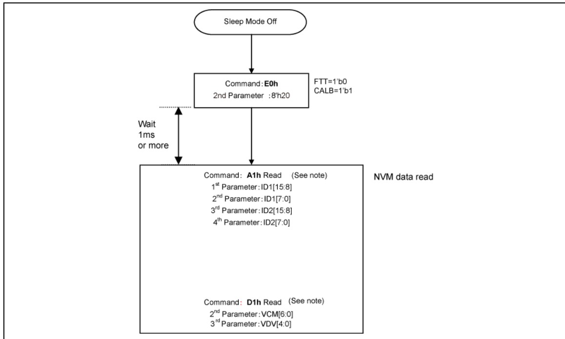
Figure 81 NVM Load (Register Resetting) Sequence
