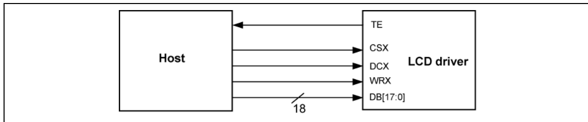
Figure 71 Interface Example for Display-Synchronous Data Transfer
