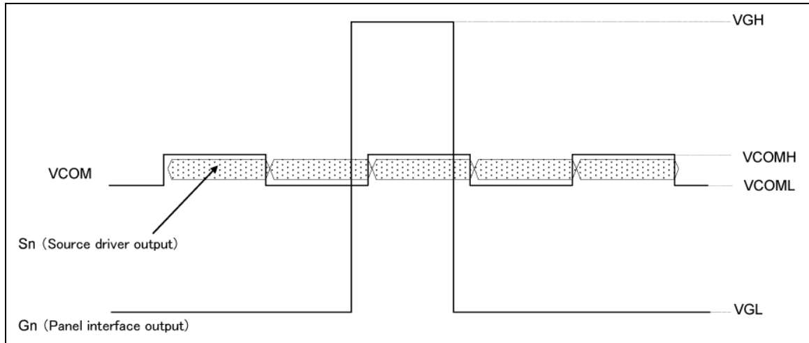
Figure 80 Voltage Applications to TFT Display
