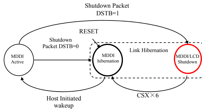
Figure 39 State Transitions in Shutdown Mode
