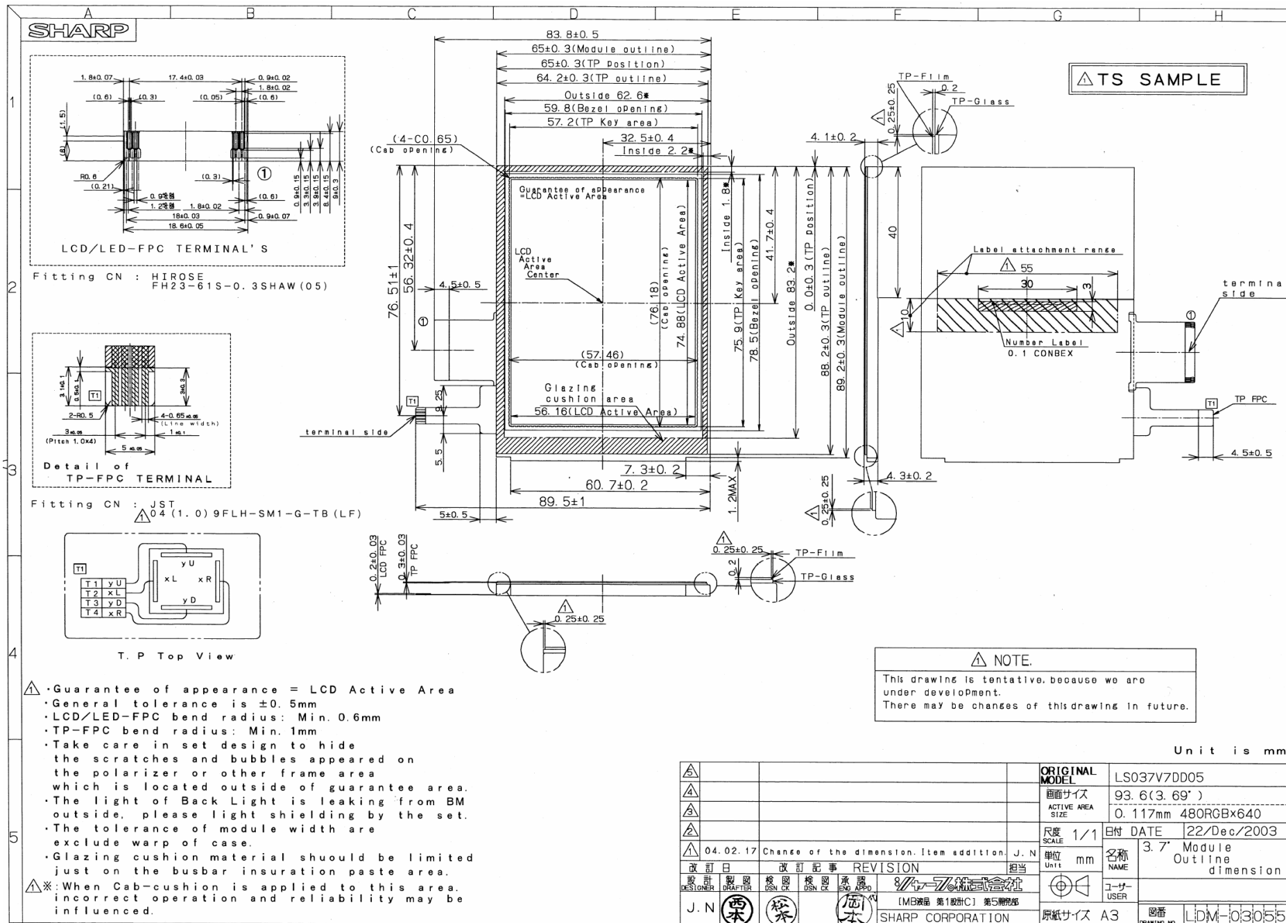
Fig.1 Outline dimensions
