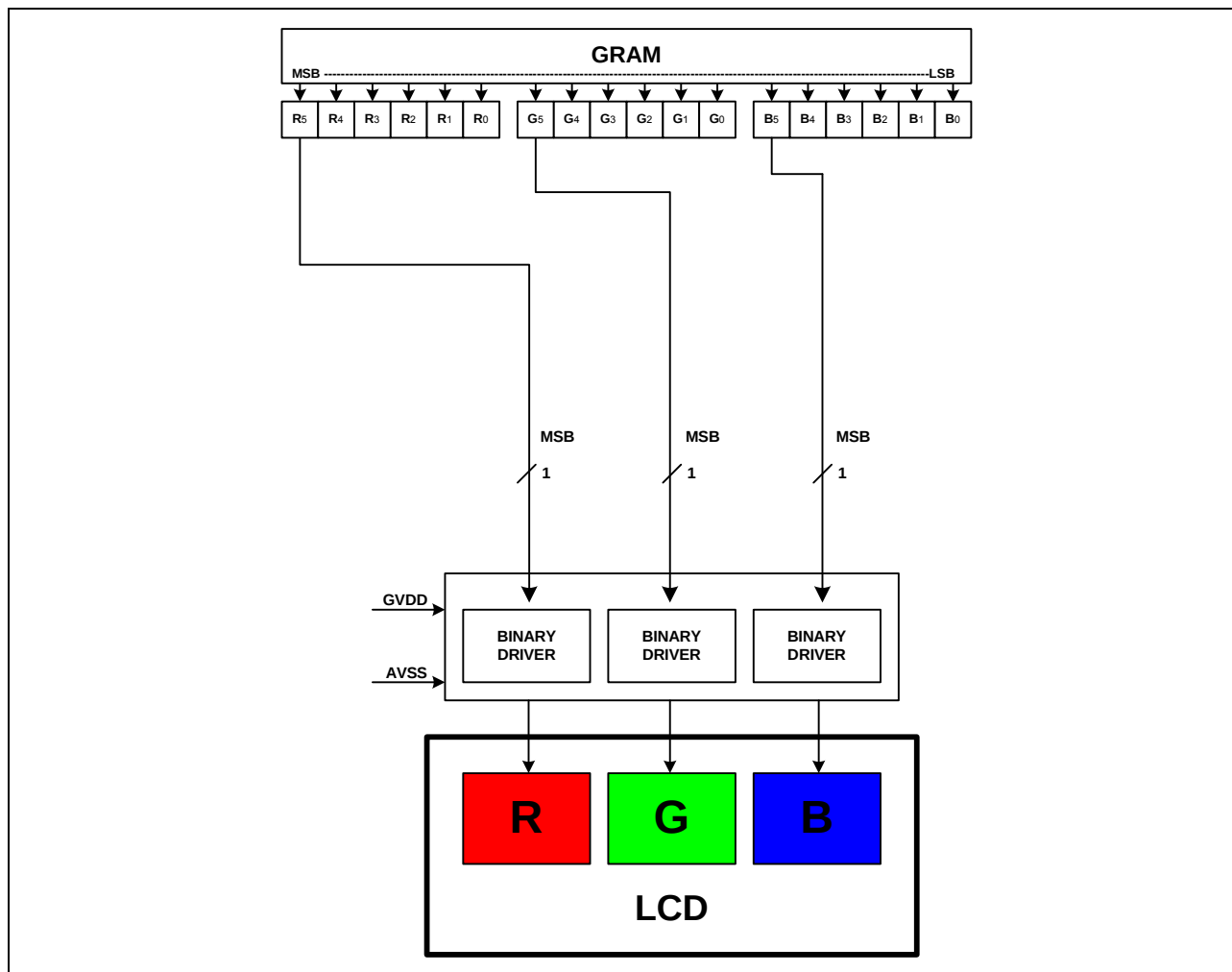
Figure 127. 8-Color Display Control
