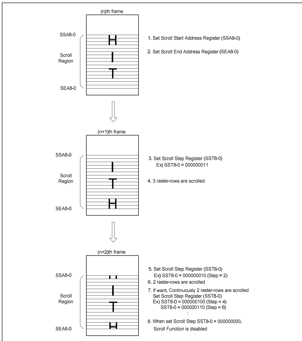
Figure 32. Vertical Scroll Display
