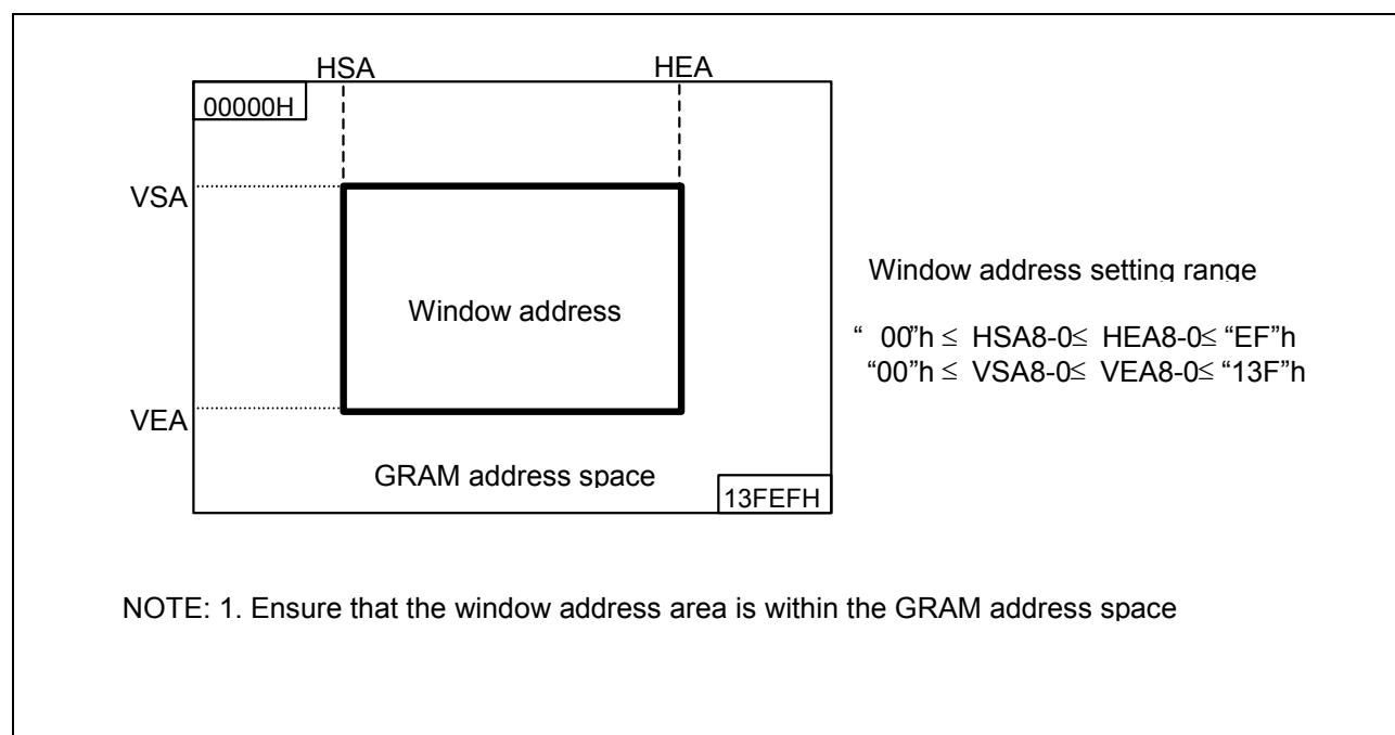
Figure 34. Window Address Setting Range (AM=0)
