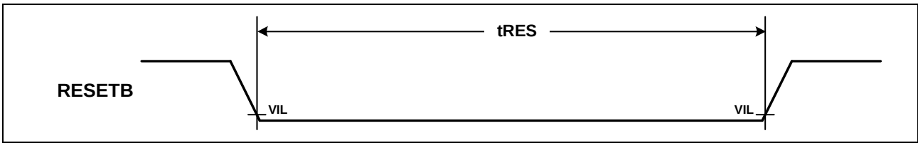
Figure 12. AC characteristics (RESET timing)
