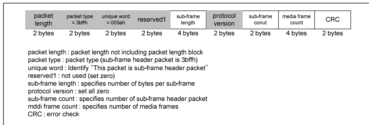
Figure 92. Sub-frame header packet structure
