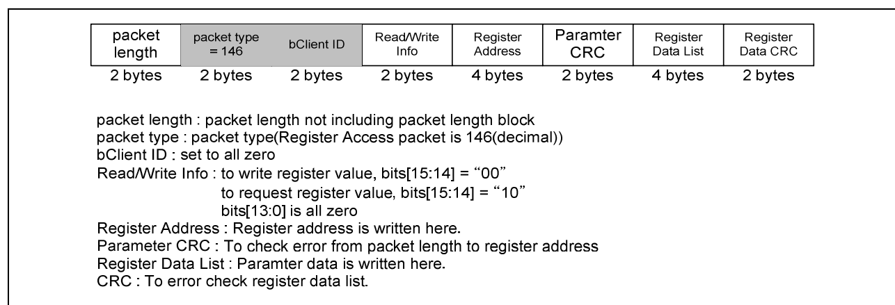
Figure 93. Register access packet structure
