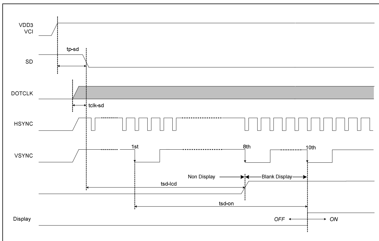
Figure 19. Power Up Sequence Timing Diagram
