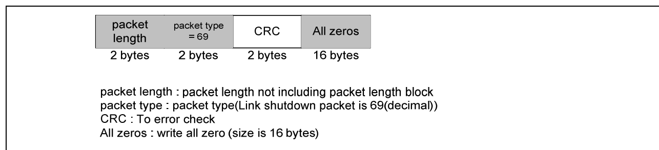
Figure 96. Link shutdown packet structure
