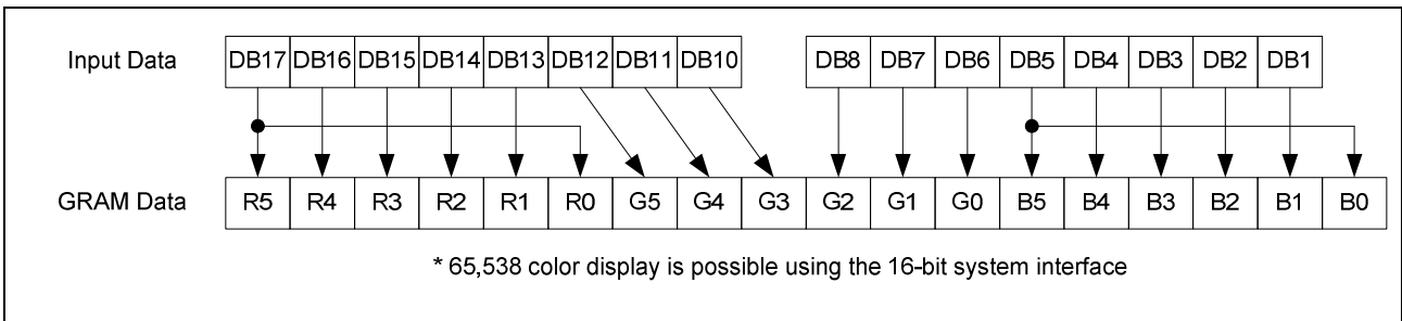
Figure 51. Bit Assignment of GRAM Data on 68-16bit CPU Interface
