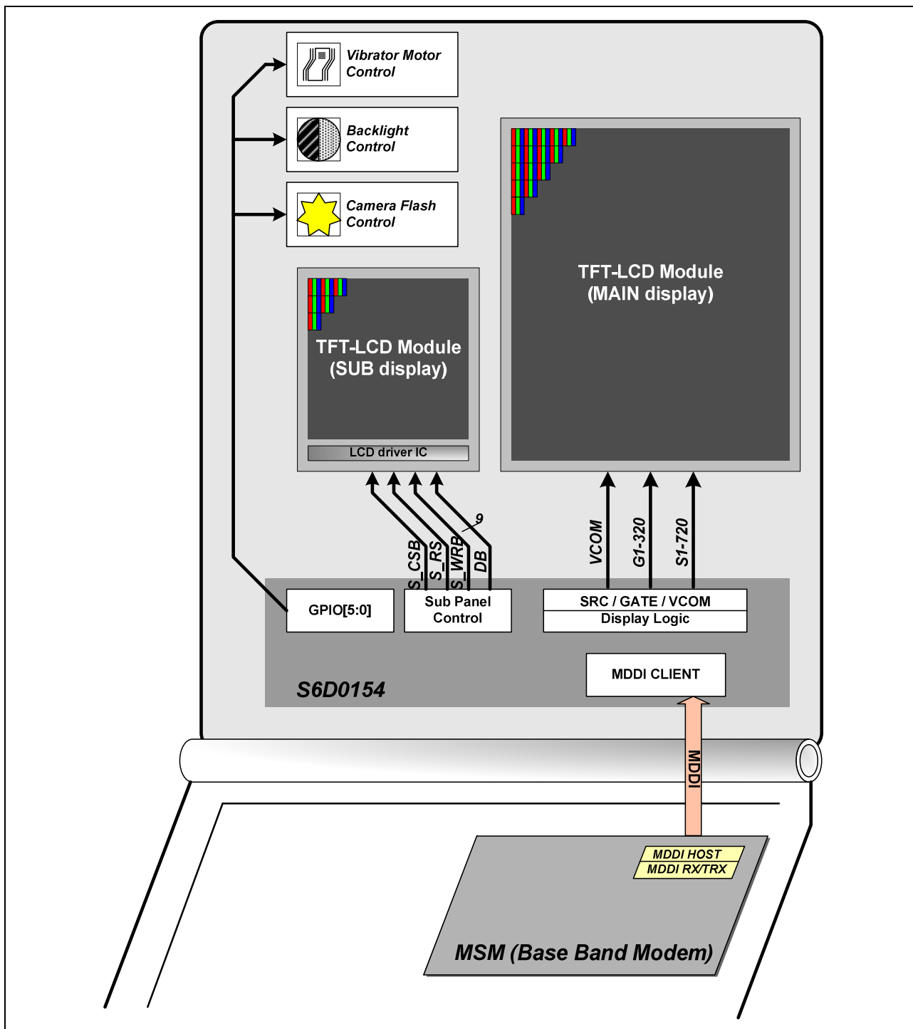
Figure 119. MDDI-integrated system structure
