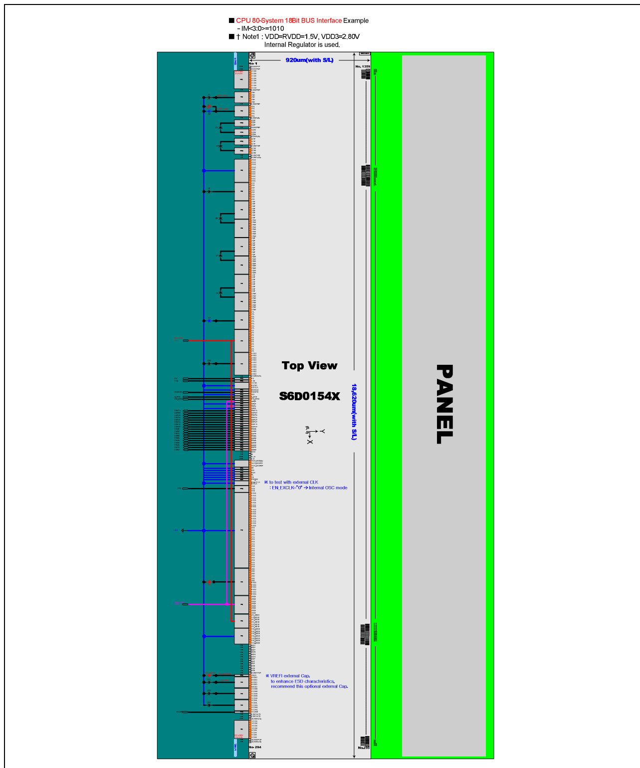
Figure 134. Application Circuit Example
