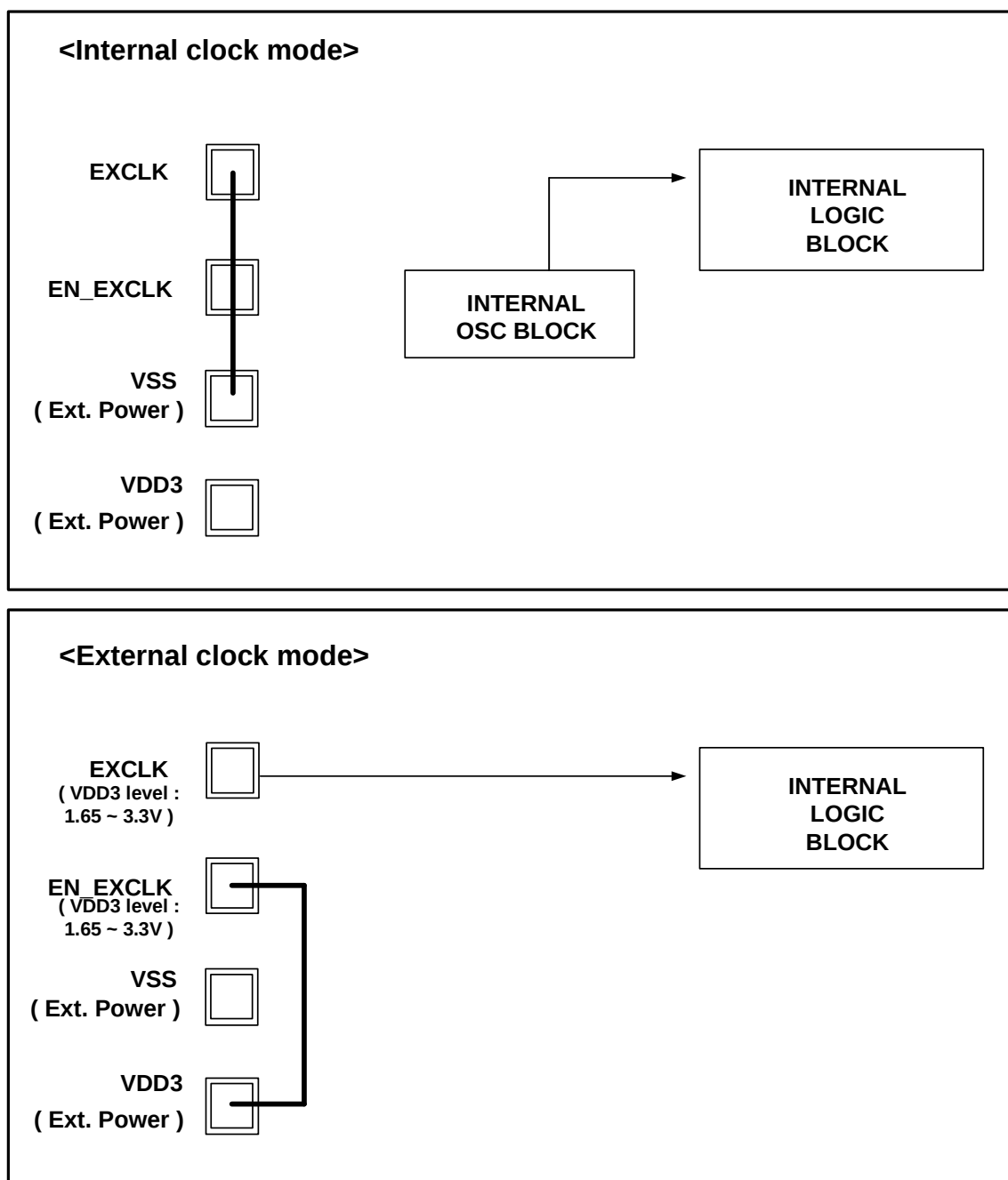
Figure 132. Oscillation Circuit
