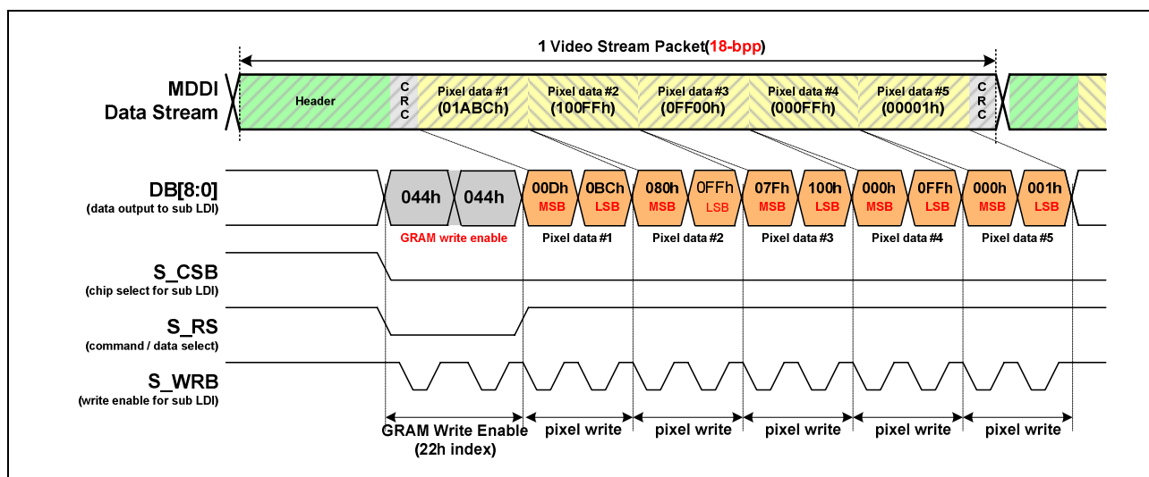
Figure 108. 80 mode 9 bit video data transfer
