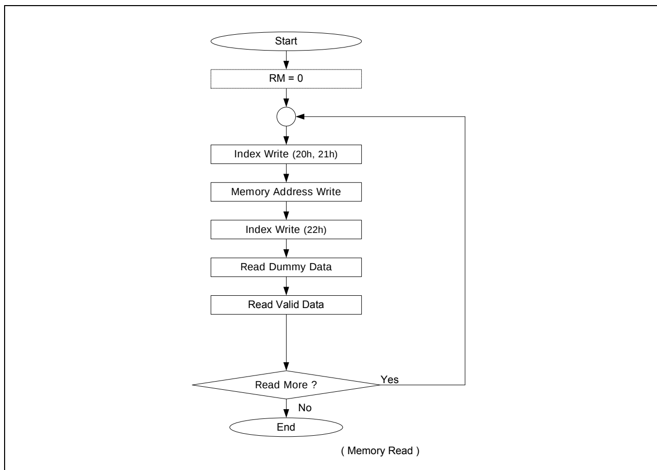
Figure 29. Memory Data Read Sequence
