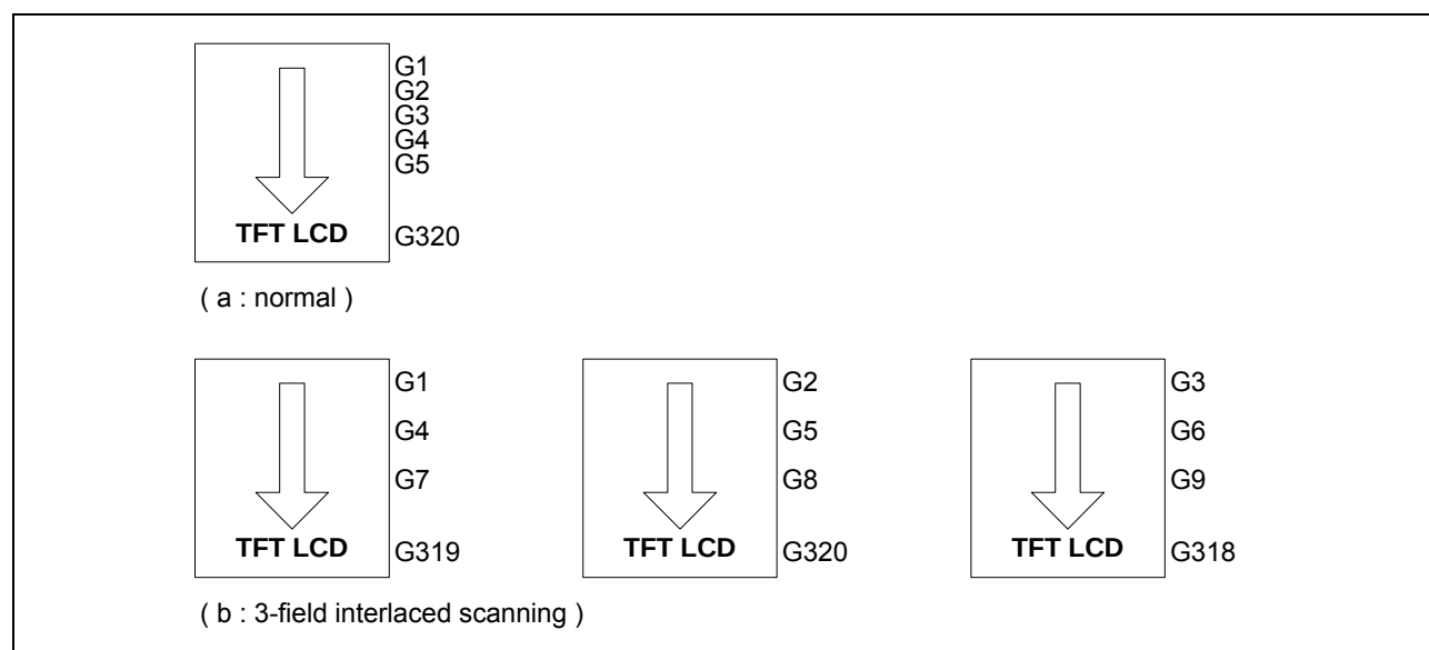
Figure 24. Interlaced scanning methods
