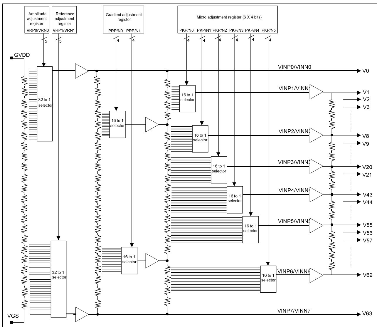
Figure 121. Structure of Grayscale Amplifier
