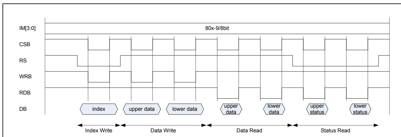
Figure 70. Timing Diagram of 80-8bit CPU Interface
