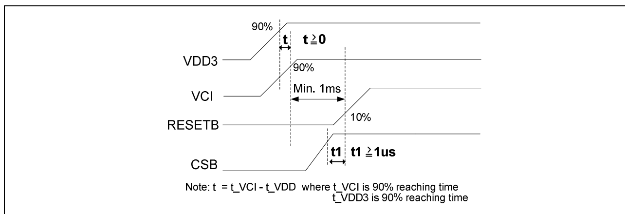
Figure 15. External power on sequence
