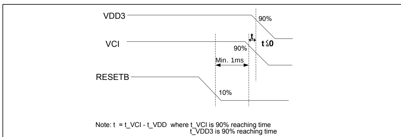
Figure 16. External power off sequence
