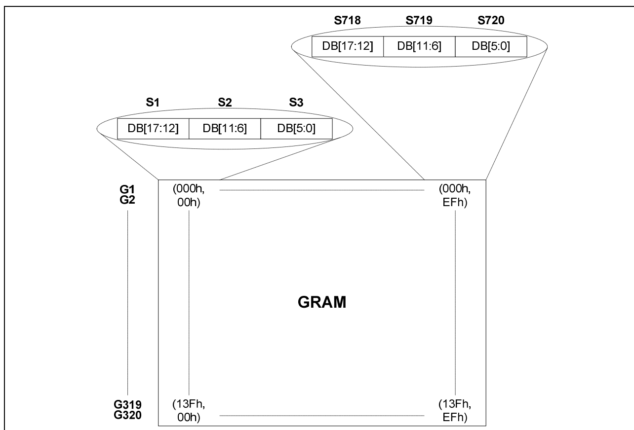
Figure 17. GRAM Address and Display Image
