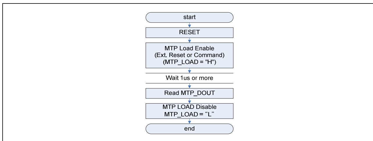
Figure 38. Flow of MTP Load / Read
