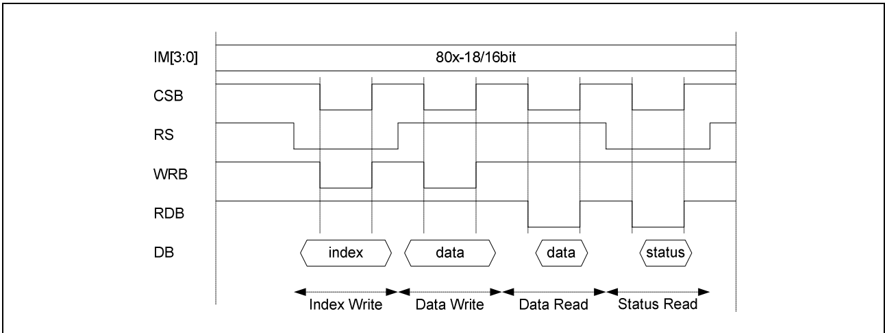
Figure 61. Timing Diagram of 80-18bit CPU Interface
