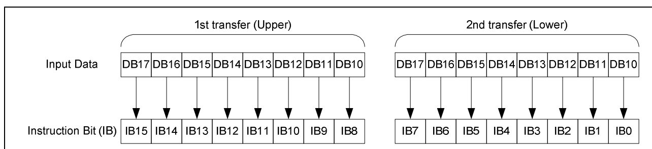
Figure 56. Bit Assignment of Instructions on 68-8bit CPU Interface
