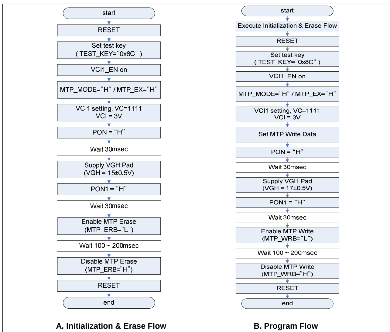
Figure 39. MTP Initialization, Erase and program
