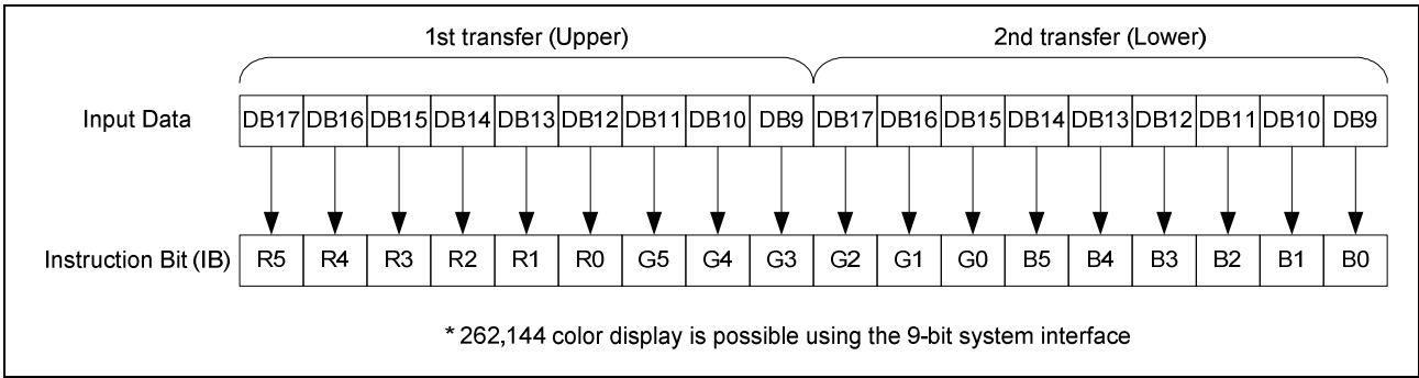
Figure 54. Bit Assignment of GRAM Data on 68-9bit CPU Interface
