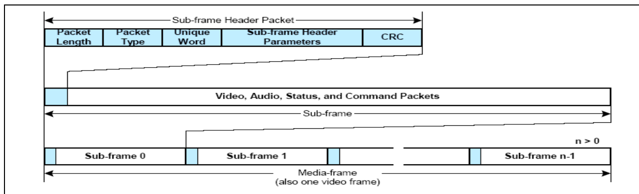
Figure 91. MDDI packet structure
