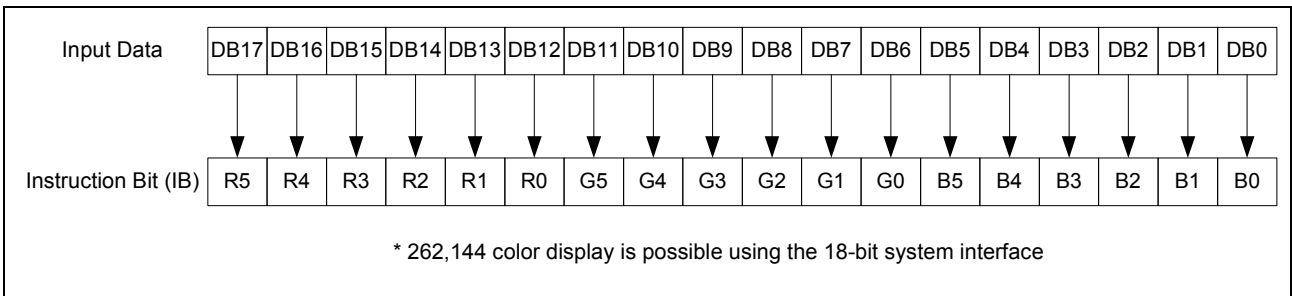
Figure 60. Bit Assignment of GRAM Data on 80-18bit CPU Interface
