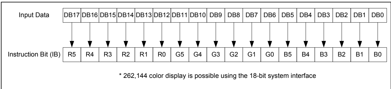
Figure 48. Bit Assignment of GRAM Data on 68-18bit CPU Interface
