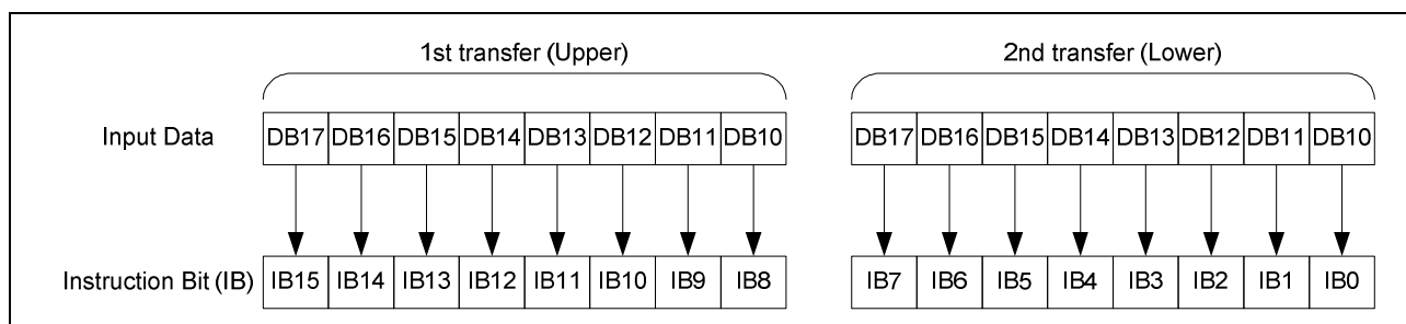
Figure 68. Bit Assignment of Instructions on 80-8bit CPU Interface
