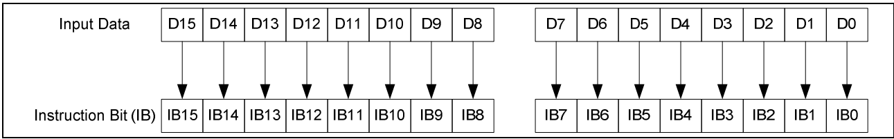
Figure 71. Bit Assignment of Instructions on SPI
