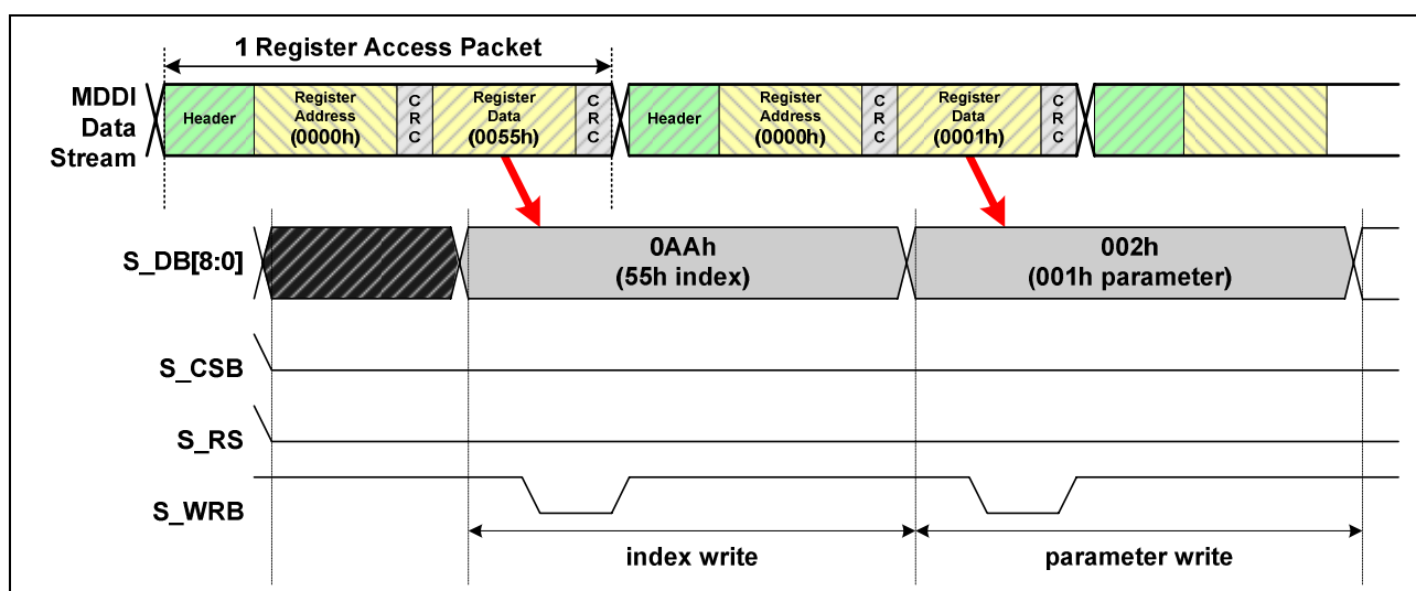
Figure 110. 80 mode STN type conventional register instruction
