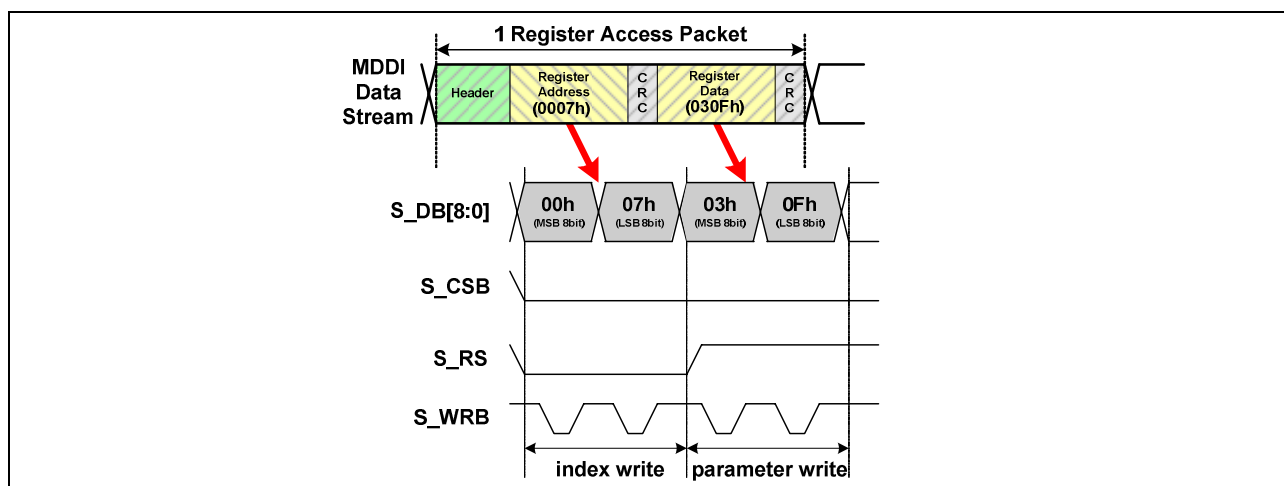
Figure 107. 80mode 9/8 bit type register access data transfer
