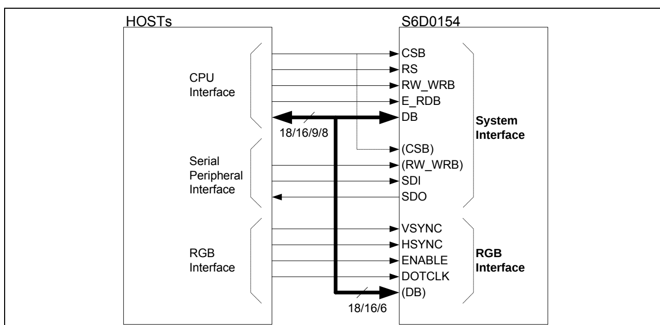
Figure 46. System Interface and RGB Interface
