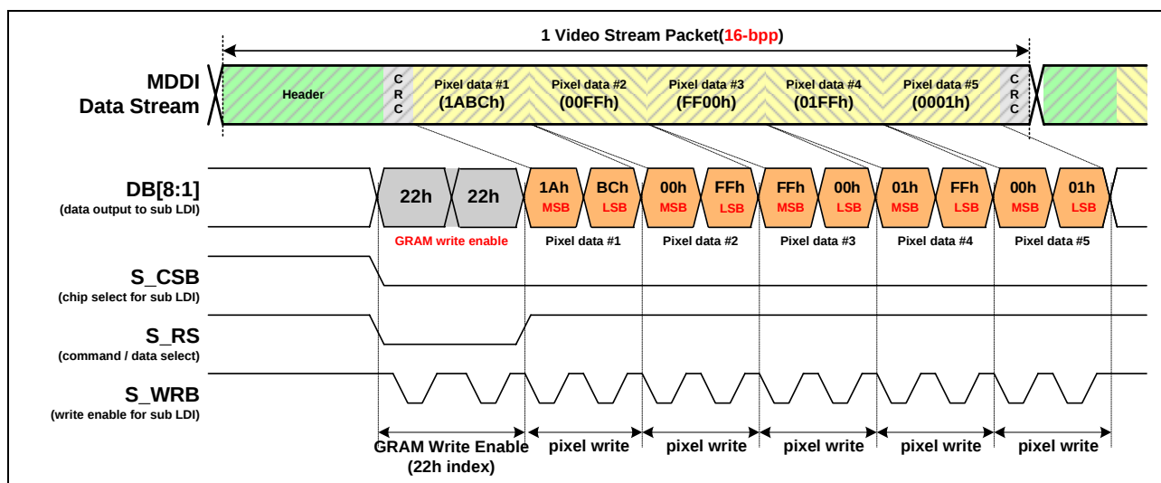
Figure 109. 80 mode 8 bit video data transfer
