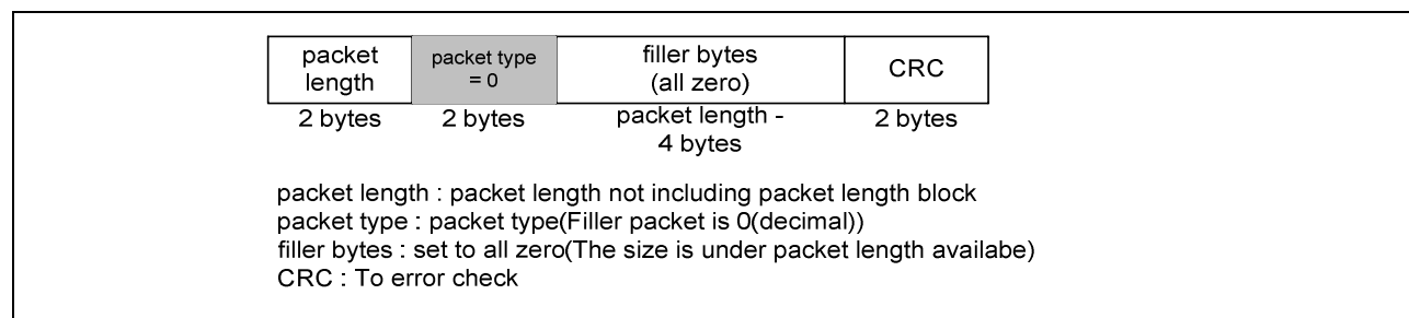
Figure 95. Filler packet structure
