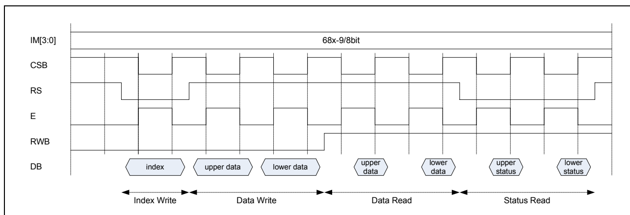
Figure 58. Timing Diagram of 68-8bit CPU Interface
