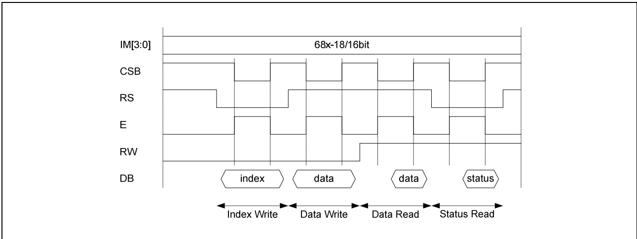
Figure 52. Timing Diagram of 68-16bit CPU Interface
