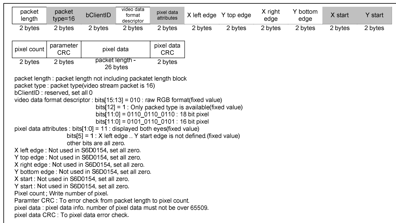
Figure 94. Video stream packet structure
