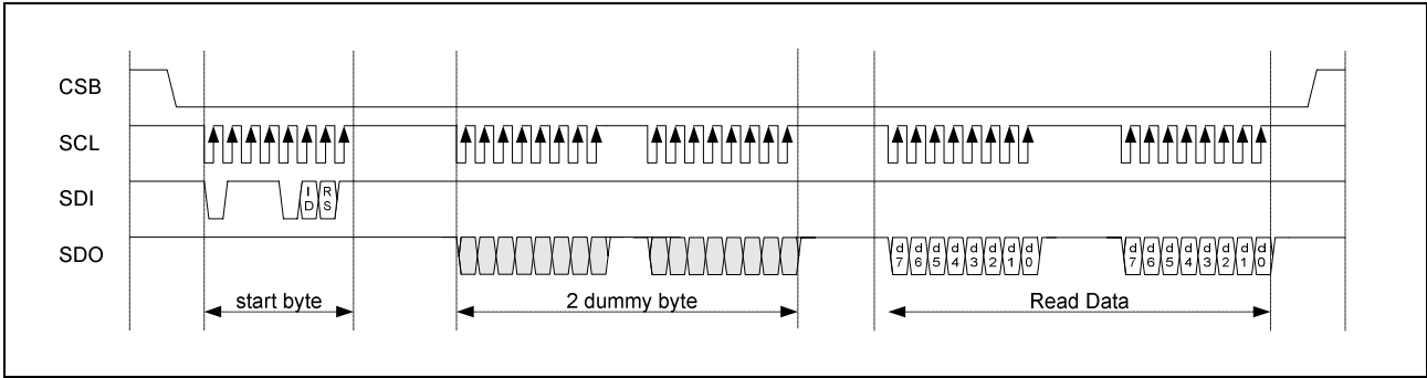
Figure 75. Timing Diagram of Register / Status Read through SPI
