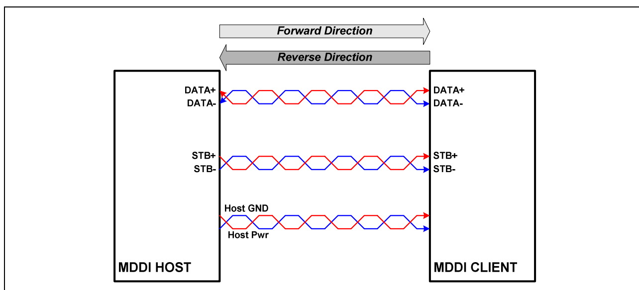
Figure 87. Physical connection of MDDI host and client
