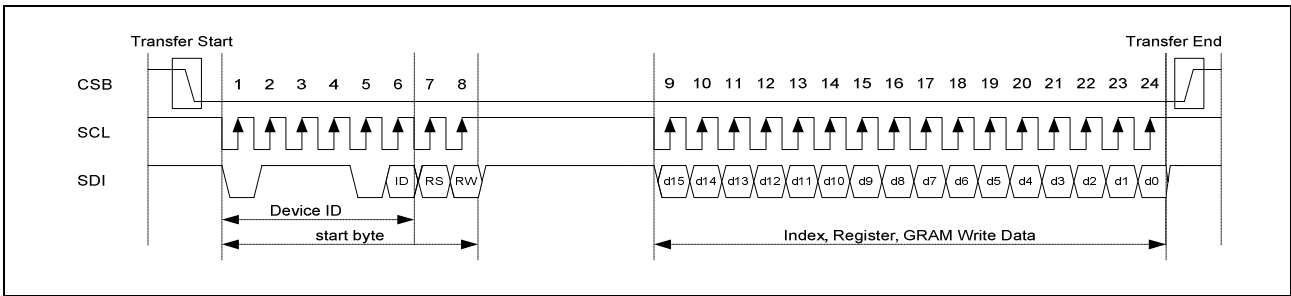
Figure 73. Basic Timing Diagram of Data Transfer through SPI
