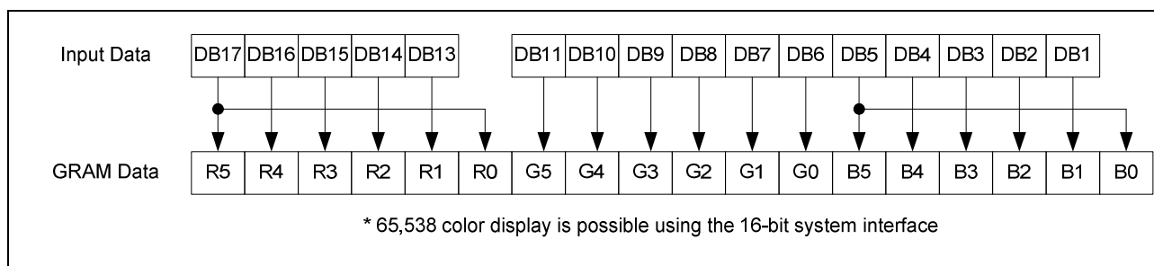
Figure 80. Bit Assignment of GRAM Data on 16bit RGB Interface
