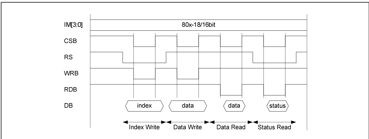
Figure 64. Timing Diagram of 80-16bit CPU Interface
