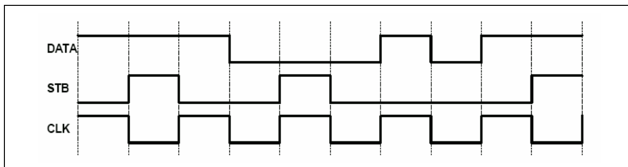
Figure 88. Data-STB encoding
