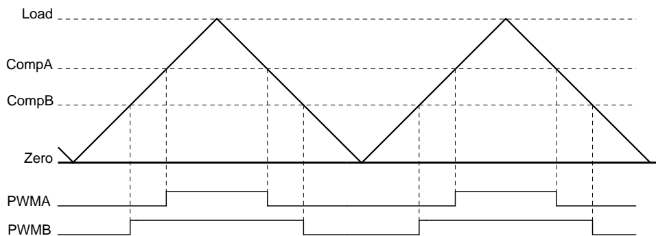
Figure 19-4. PWM Generation Example In Count-Up/Down Mode
