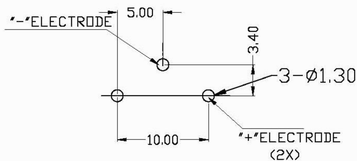
PCB LAYOUT
