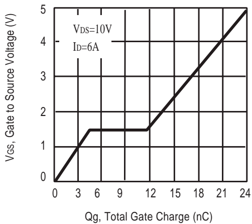
Figure 9. Gate Charge
