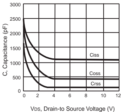
Figure 3. Capacitance
