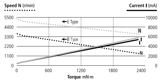
HN54, 75mm
