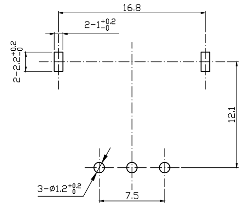
PCB TERMINAL POSITION
