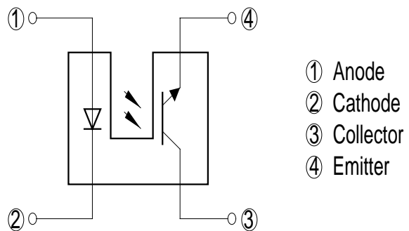
Internal connection diagram (Common to 4 models )
