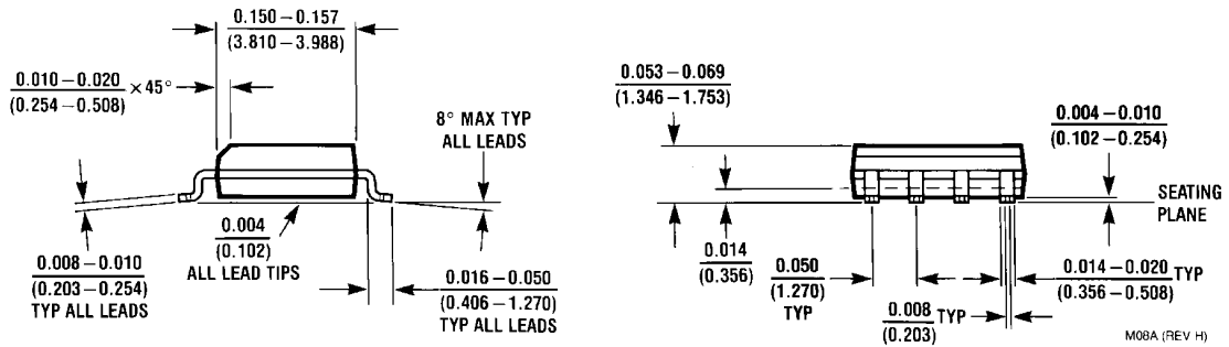
SOIC Package NS Package Number M08A
