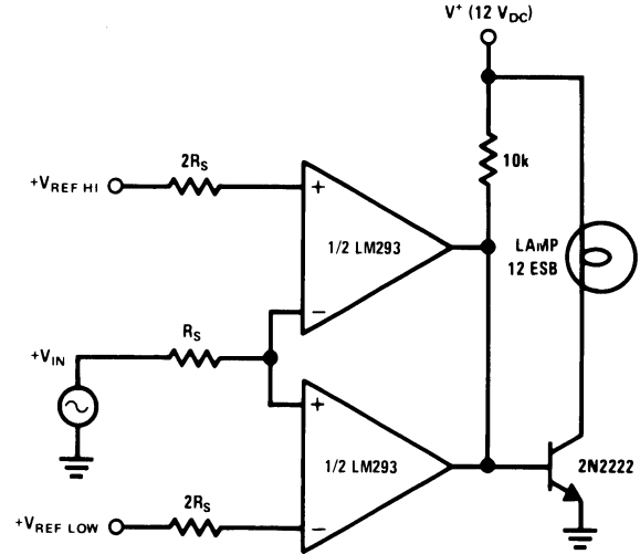
Limit Comparator
