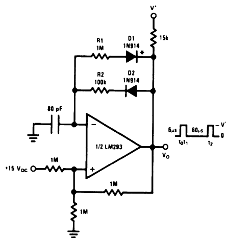
Pulse Generator
