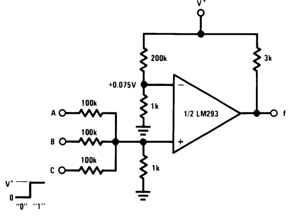
OR Gate
