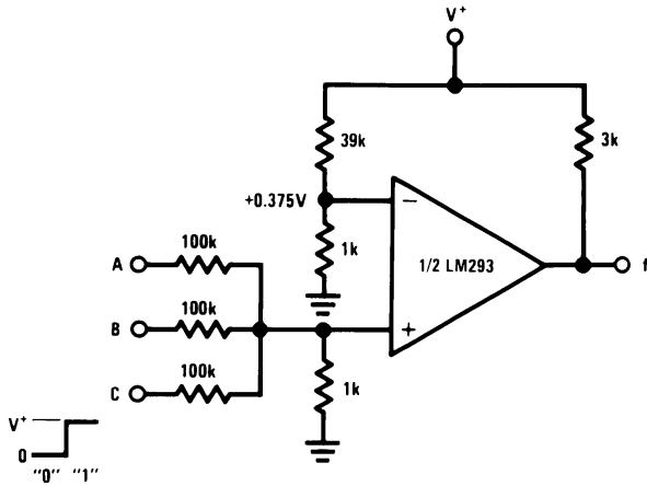
AND Gate
