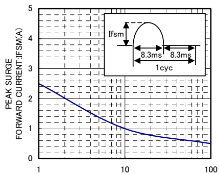
IFSM-CYCLE CHARACTERISTICS
