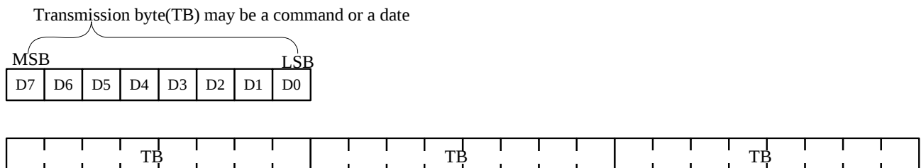
Figure2: 4-pins Serial Data Stream Format
