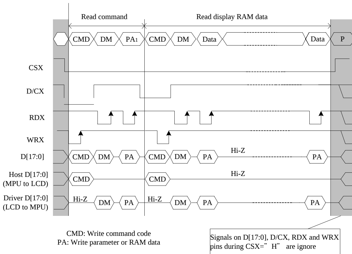
Figure12: 8080-Series parallel bus protocol (Read from register or display RAM)
