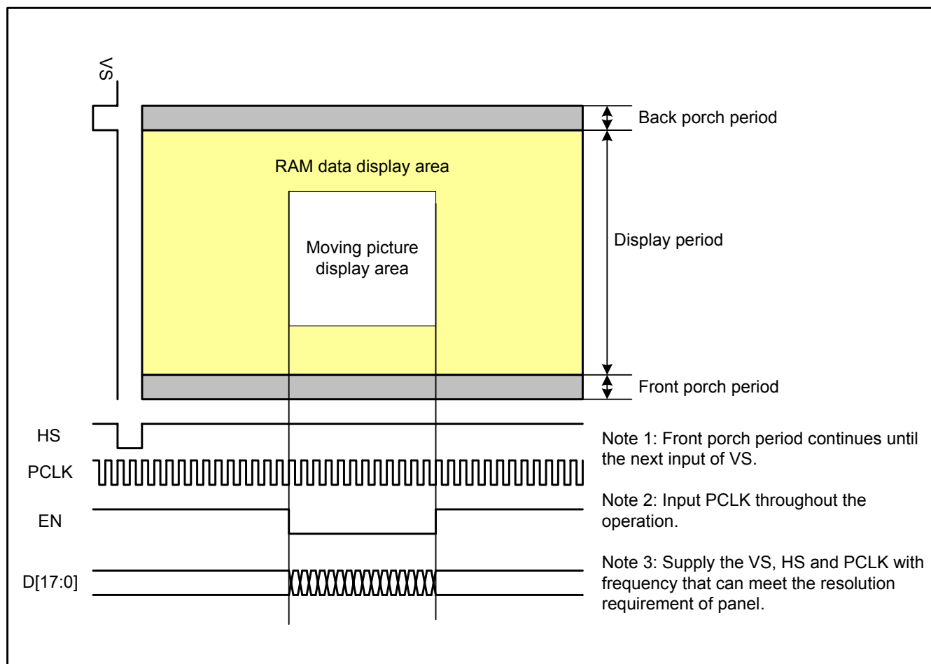
Figure23: GRAM Access Area by RGB Interface
