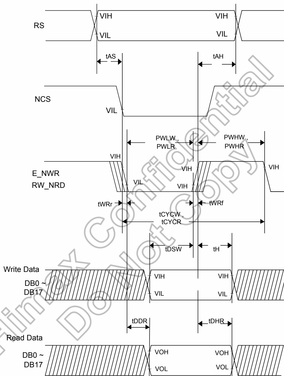
Figure 8. 1 80-system Bus Timing
