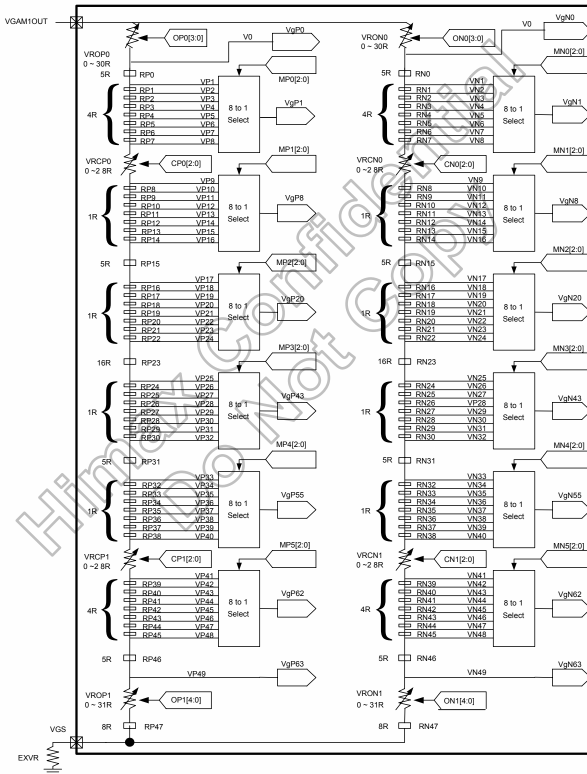
Figure 5. 22 Gamma Resister Stream and Gamma Reference Voltage
