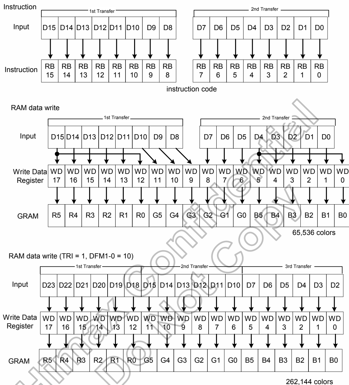
Figure 4. 13 Data Format of Serial Data Transfer Interface GRAM
