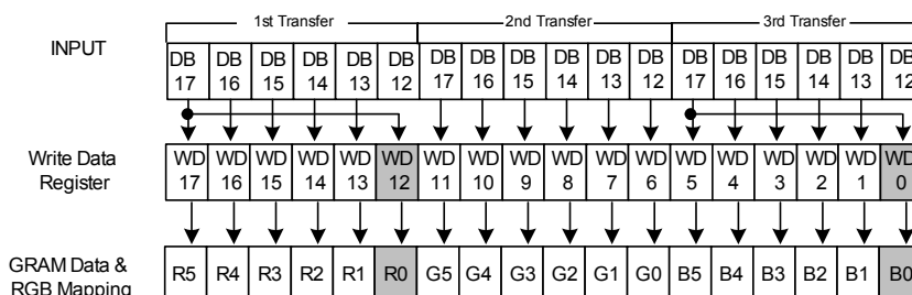
Figure 6. 32 Input Data Written to GRAM through Write Data Register in 8-bit Interface Mode
