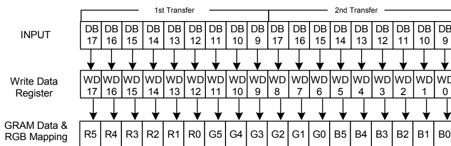
Figure 6. 31 Input Data Written to GRAM through Data Register in 9-bit Interface Mode
