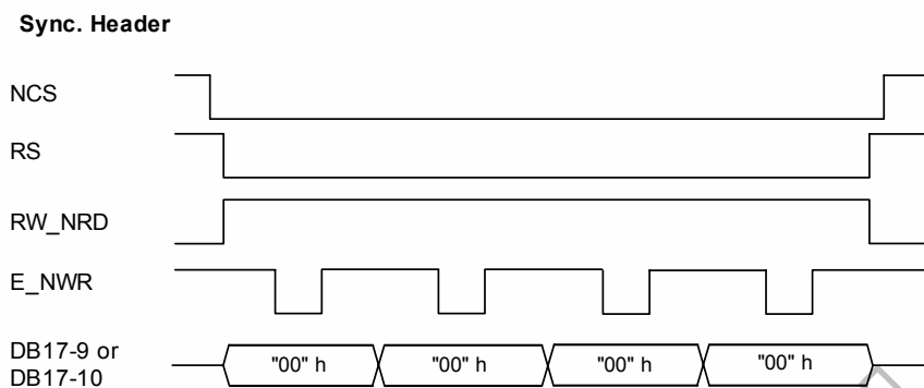
Figure 4. 12 Sync. Header for 9/8-bit Parallel Bus Interface Timing (for i80 series MPU)
