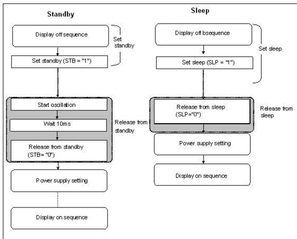
Figure 7. 5 Standby Mode and Sleep Mode Setting Sequence
