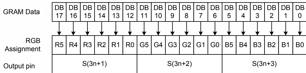
Figure 5. 1 GRAM Data and Display Data of 80-system 18-bit Bus Interface (SS = "0", BGR = "0")
