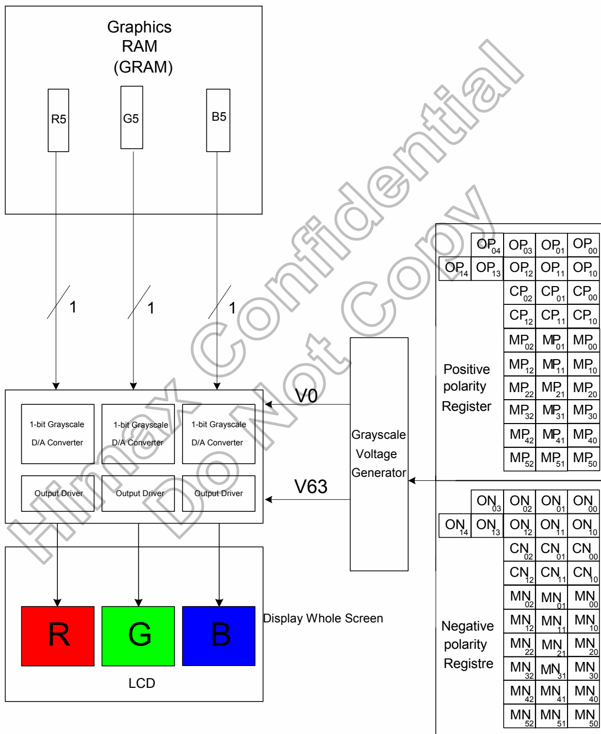
Figure 5. 15 Grayscale Control in 8-Color Mode
