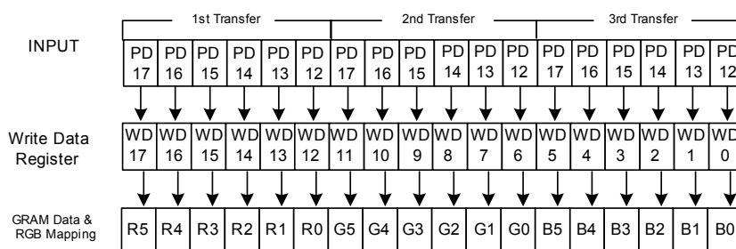
Figure 6. 33 Input Data Written to GRAM through Write Data Register in 18-/16-/6-bit RGB Interface Mode
