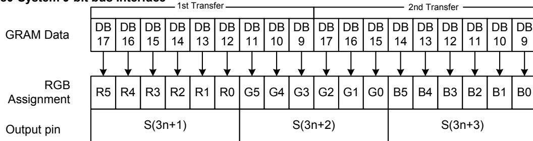
Figure 5. 3 GRAM Data and Display Data of 80-system 9-bit Bus Interface (SS = "0", BGR = "0")
