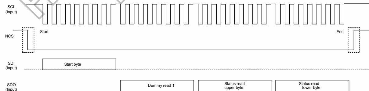
Figure 4. 14 Data Transfer through Serial Data Transfer Interface
