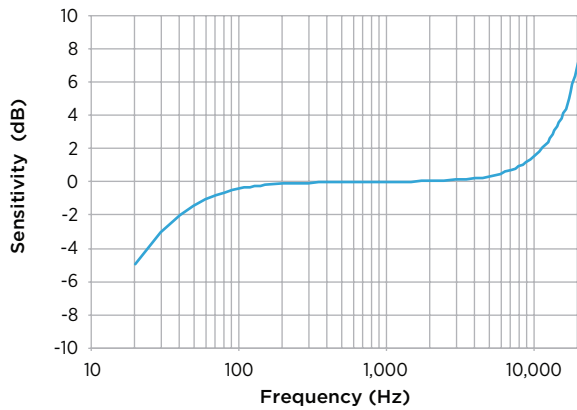
Figure 7: Typical Free Field Response Normalized to 1 kHz
