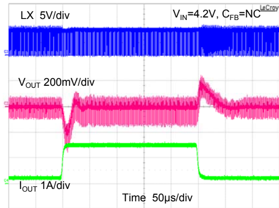
200mA ~ 1.5A Load Transient Waveform
