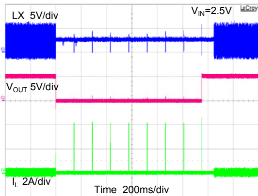
Short Circuit Waveform
