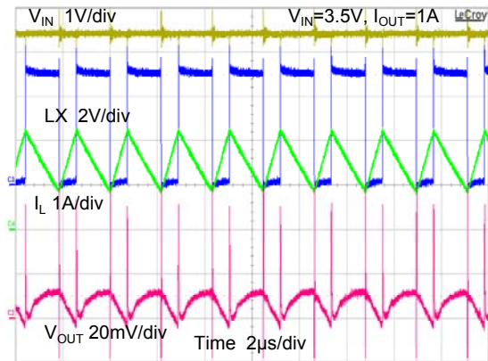
V_{IN}, V_{OUT}, I_L Waveform
