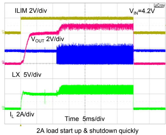
Start Up Waveform
