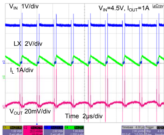
V_{IN}, V_{OUT}, I_L Waveform
