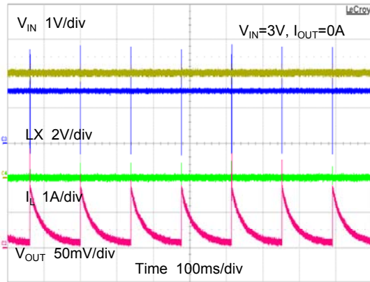
V_{IN}, V_{OUT}, I_L Waveform
