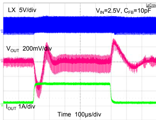
200mA ~ 1.5A Load Transient Waveform
