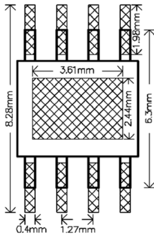
SOP-8 (FD)
