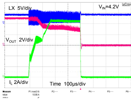
Over Current & Under Voltage Waveform
