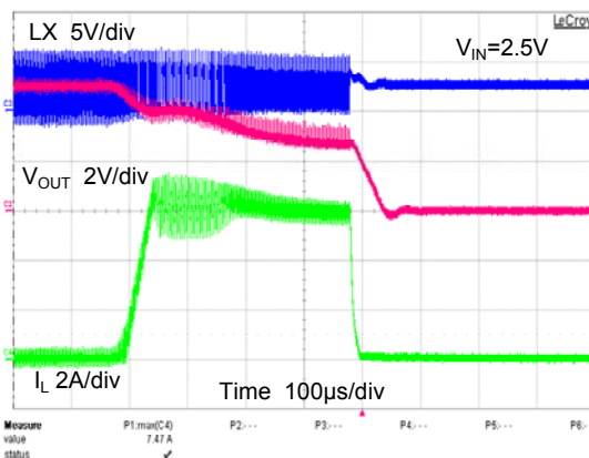
Over Current & Under Voltage Waveform
